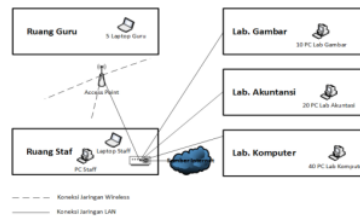
Gambar 8. Denah Ruangan
