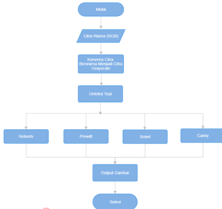
1 Gambar 1. Proses Deteksi Tepi Citra Digital
