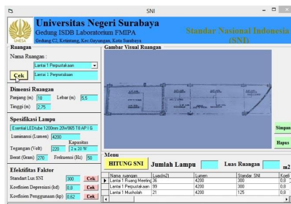
Gambar 5. Program perhitungan standar lampu
