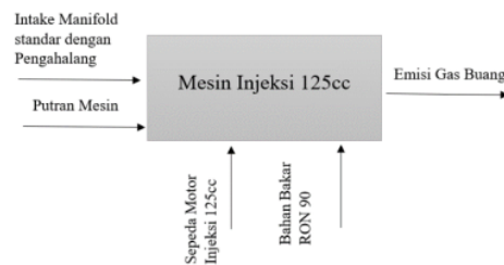
Gambar 3.1 Variabel Penelitian
