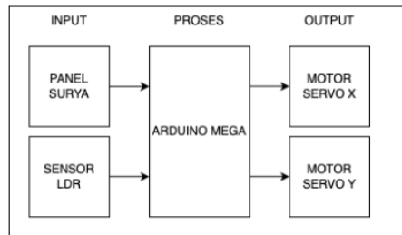
Gambar 1 Blok Diagram
