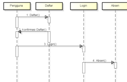
Gambar 3. Sequence Diagram
