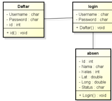
Gambar 4. Class Diagram
