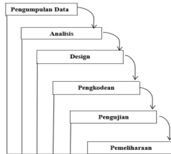
Gambar 1. Metode Waterfall
