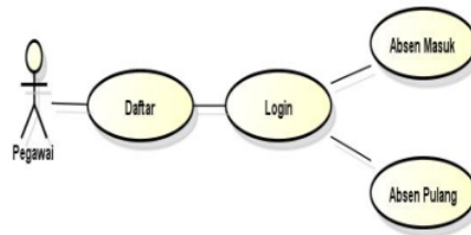
Gambar 2. Usecase Diagram
