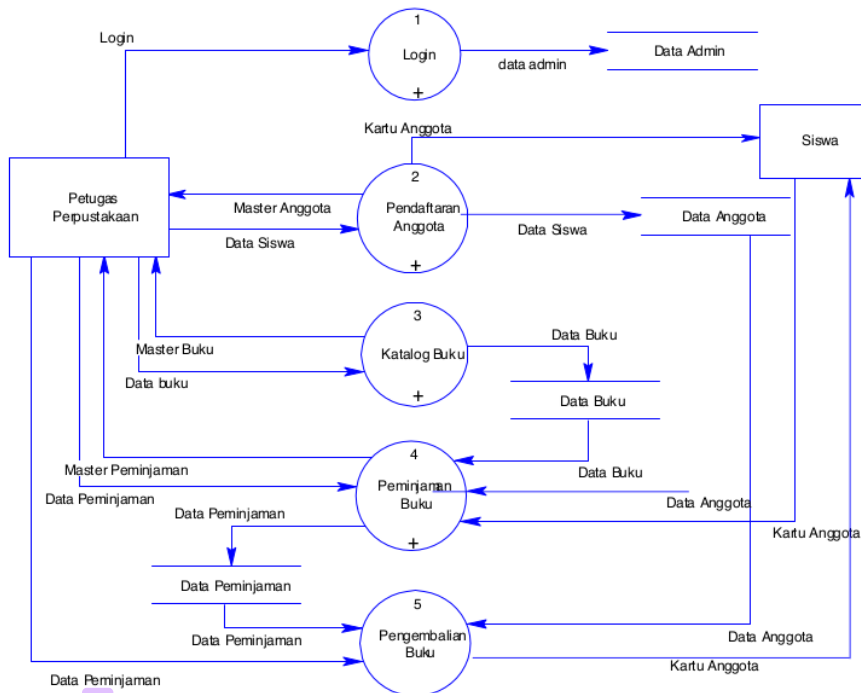
Gambar 4 Data Flow Diagram Level 0
