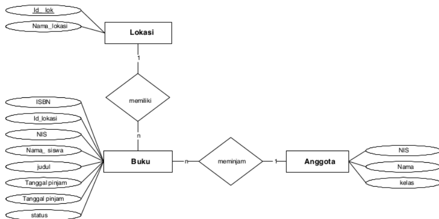
Gambar 9 ERD (Entity Relationship Diagram)
