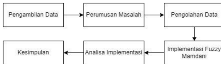
Gambar 1. Alur Penelitian
