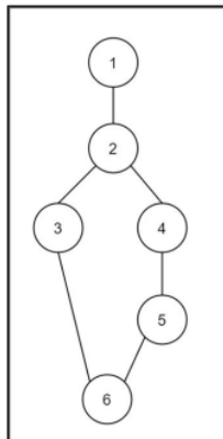
Gambar 4.1 Flowgraph Menu Stok Barang
