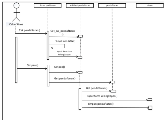
Gambar 5. Sequence Diagram siswa
