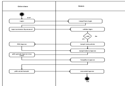
Gambar 10. Activity Diagram Laporan Formulir Pendaftaran
