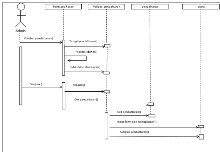
Gambar 6. Sequence Diagram Halaman Admin
