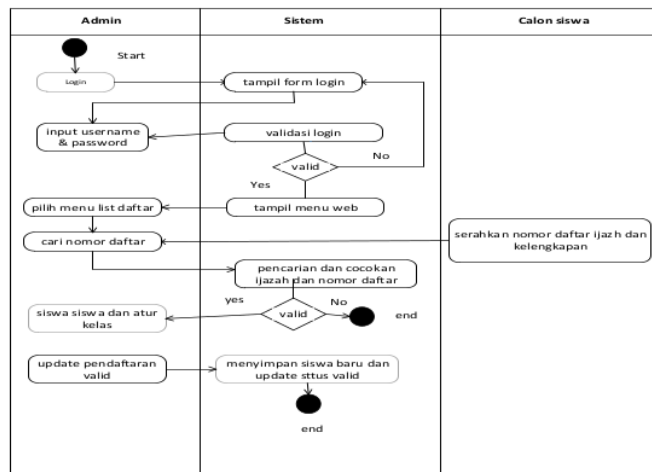
Gambar 11. Activity Diagram Admin Memferivikasi Data
