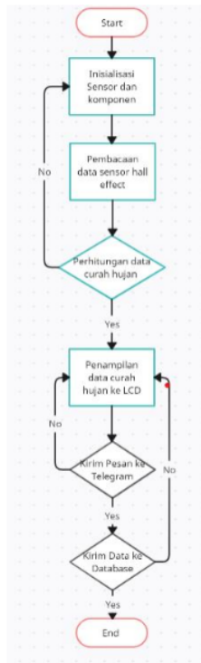
Gambar 5. Flowchart
