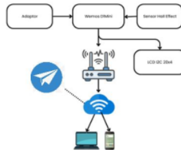
Gambar 4. Diagram blok
