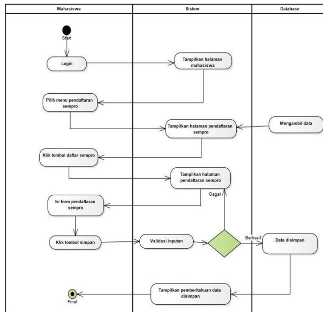
Gambar 4. Activity diagram pendaftaran sidang proposal
