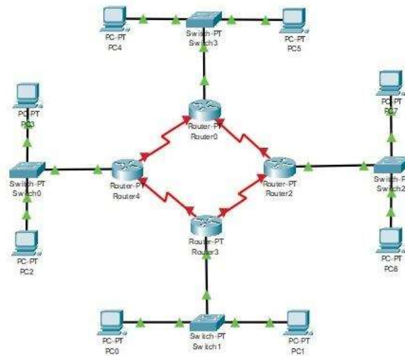
Gambar 1. Topologi Ring
