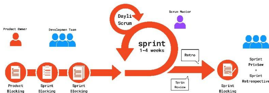
Gambar 3. Scrum
