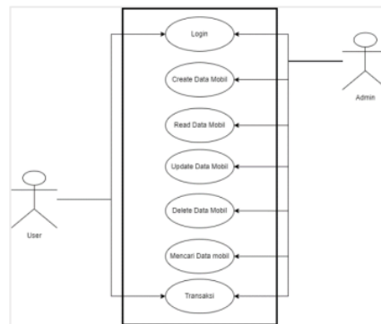
7 Gambar 1. Use Case Diagram sistem rental mobil
