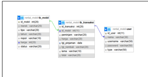
Gambar 2. Entity Relationship Diagram
