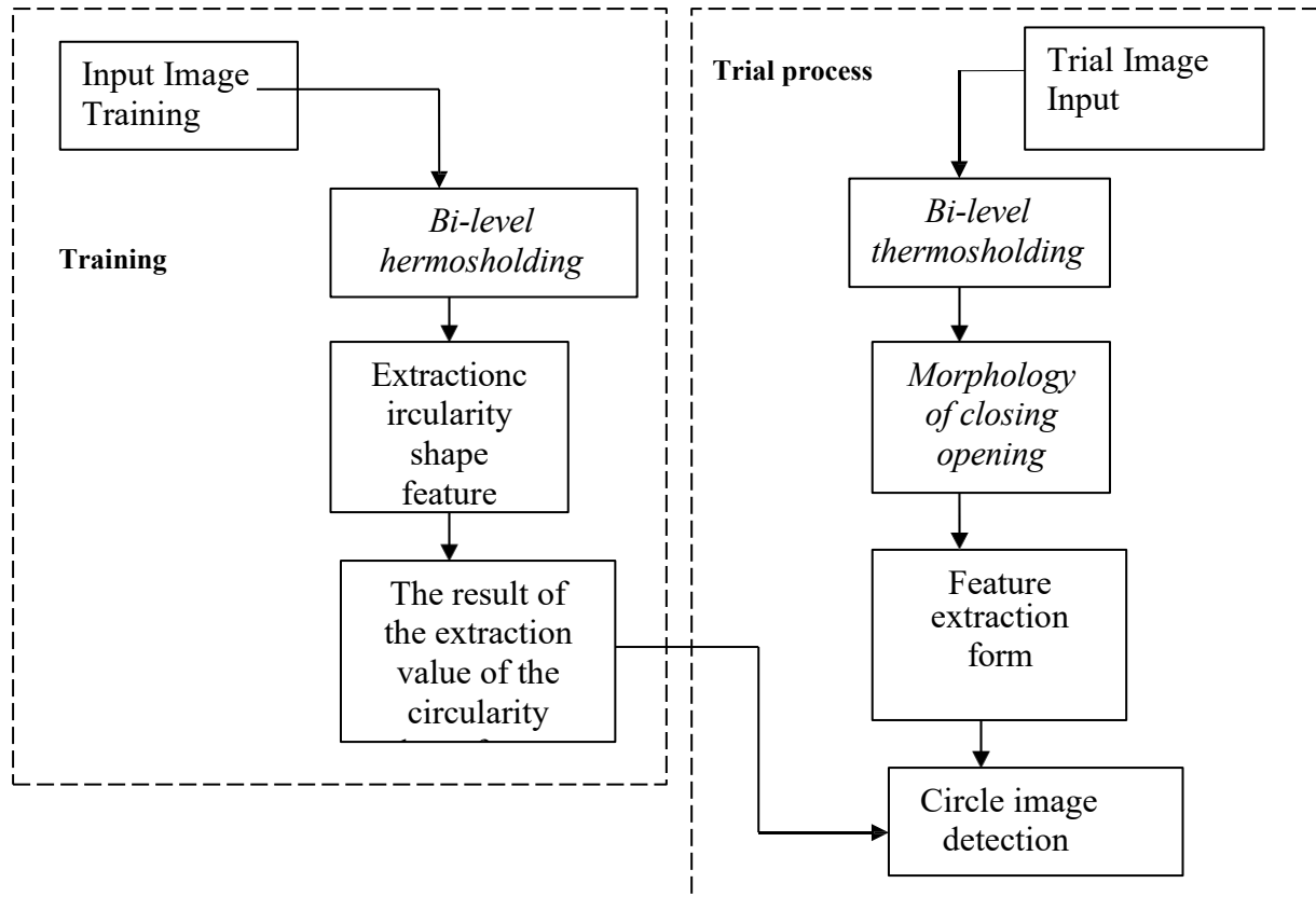
Figure 2. Diagram of the circle image detection system
