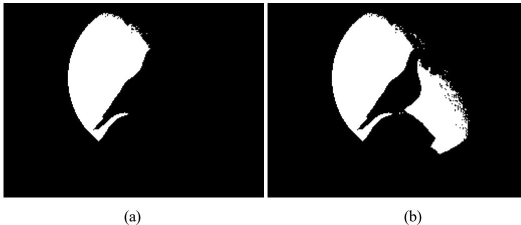
Figure 6. (a) segmented image, (b) image after morphological closing and opening process.
