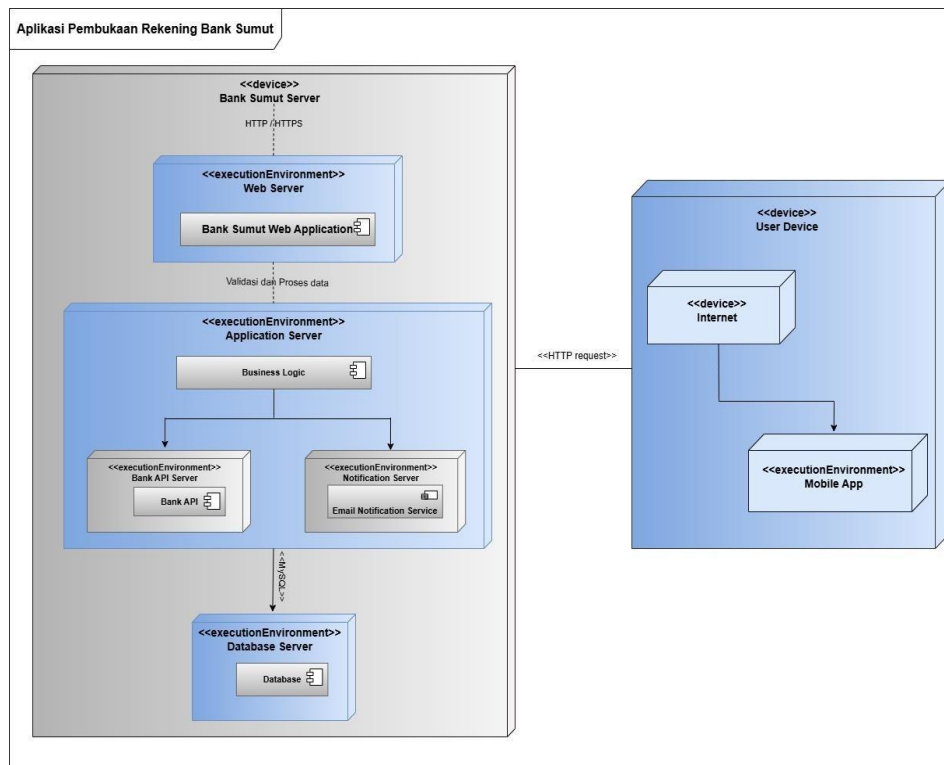
Gambar 3.6 Deployment Diagram
