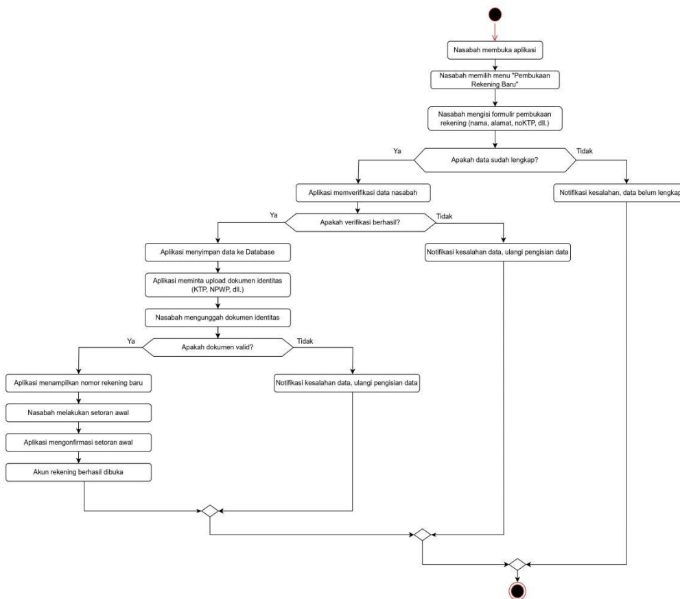
Gambar 3.3 Activity Diagram
