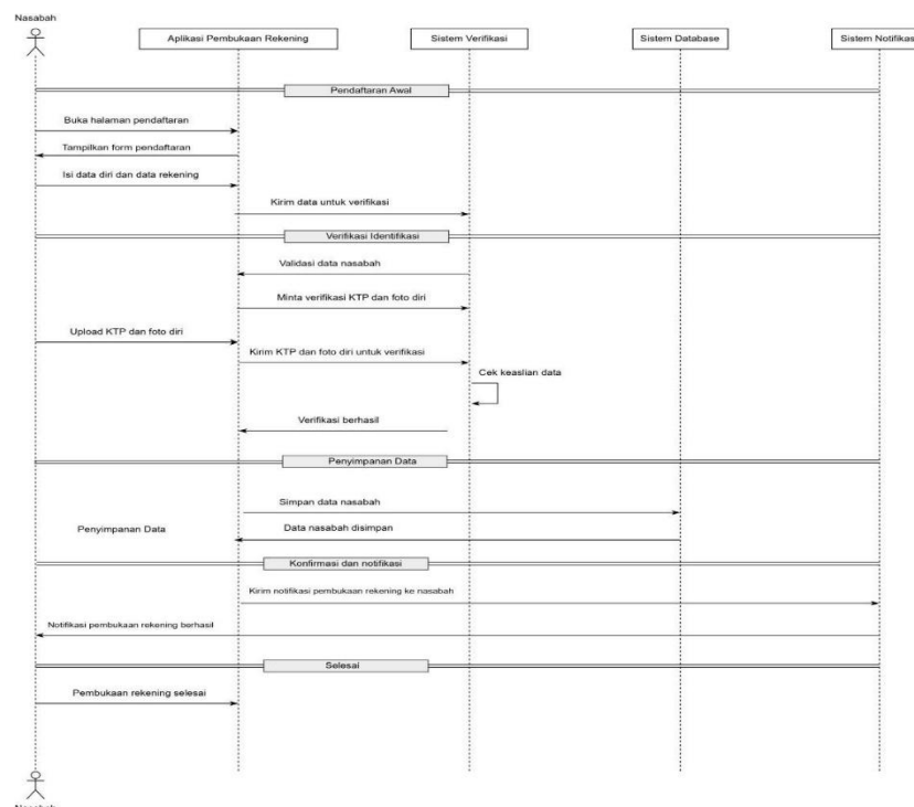
Gambar 3.4 Sequence Diagram
