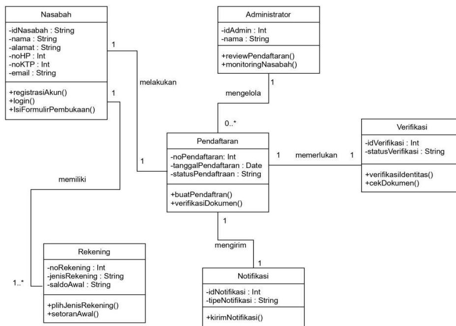
Gambar 3.2 Class Diagram
