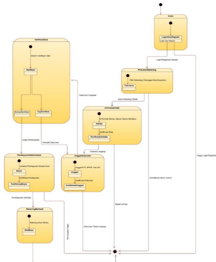
Gambar 3.5 State Diagram
