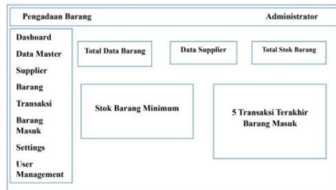
Gambar 6. Dashboard
