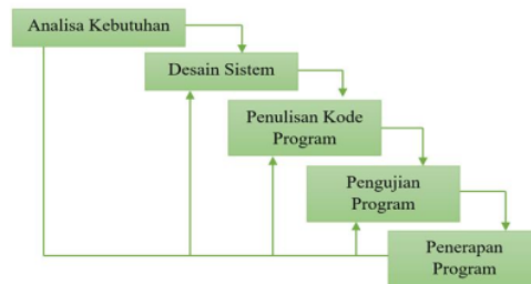
Gambar 1. Model Waterfall
