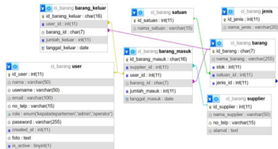
Gambar 4. Diagram Logical Record Structure
