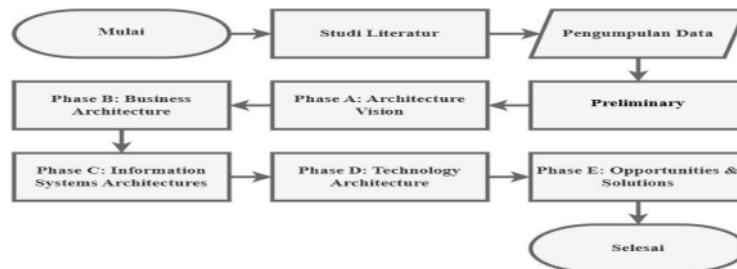
Gambar 1. Flowchart penelitian
