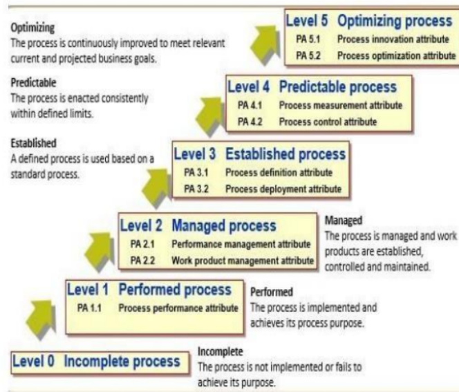
Gambar 1. Proses Level Kapabilitas (ISACA, 2013)
