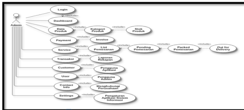
Gambar 2. Use Case Diagram Admin
