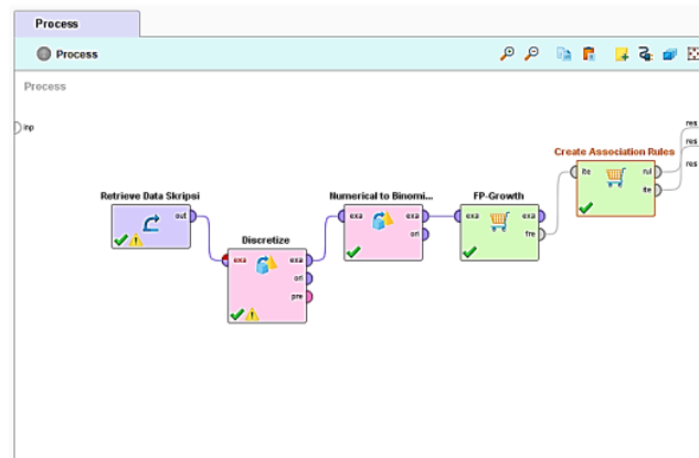
Gambar 5. Susunan Operator Asosiasi
