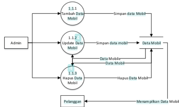
Gambar 4. DFD Level 2 Proses 1.1
