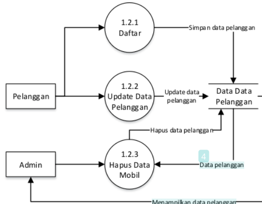
Gambar 5. DFD Level 2 Proses 1.2
