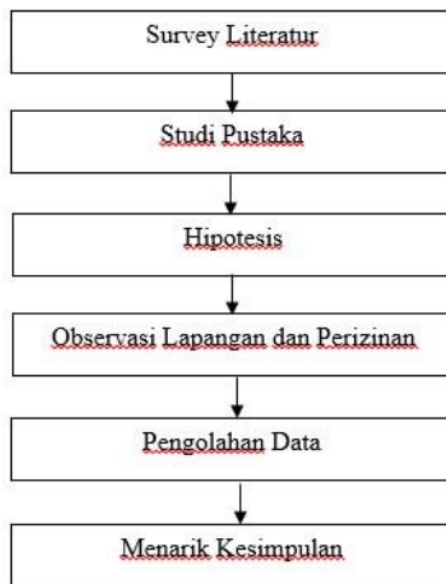
Gambar III.1 Konsep Penelitian
