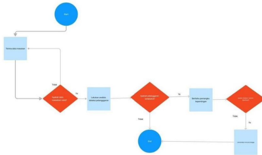
Gambar 2 Flowchart fitur Breach Monitor
