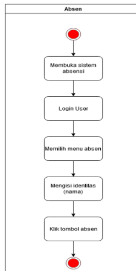
Gambar 3. Activity Diagram
